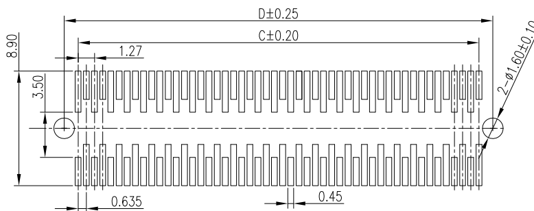
RECOMMENDED PCB LAYOUT(TOP SIDE) PCB BOARD TOLFRANCF±0.05
