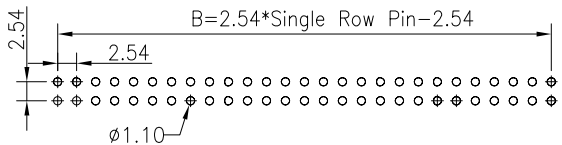
Recommended P.C.B Layout (Top Side) (PCB BOARD TOLFRANCF+0.05)
