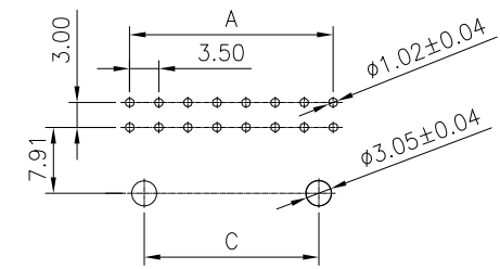
PCB LAYOUT (2*4~2*8)
