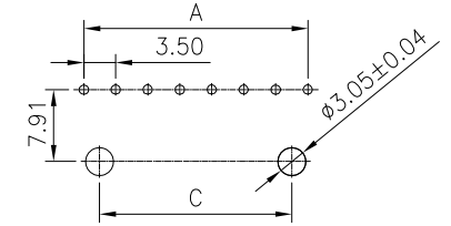
PCB LAYOUT (4~8PRI)
