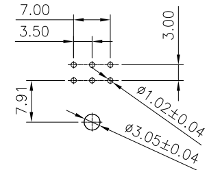
PCB LAYOUT (2*2~2*3)
