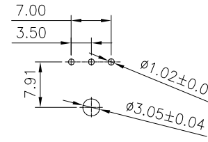
PCB LAYOUT (2~3PRI)
